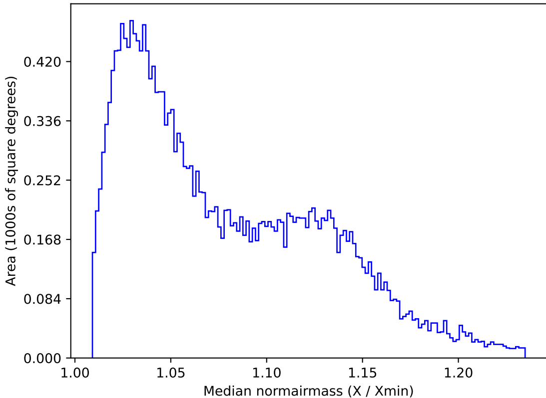
too_elab_r32_d3_giz_v3.4_10yrs All sky u band: Median normairmass
