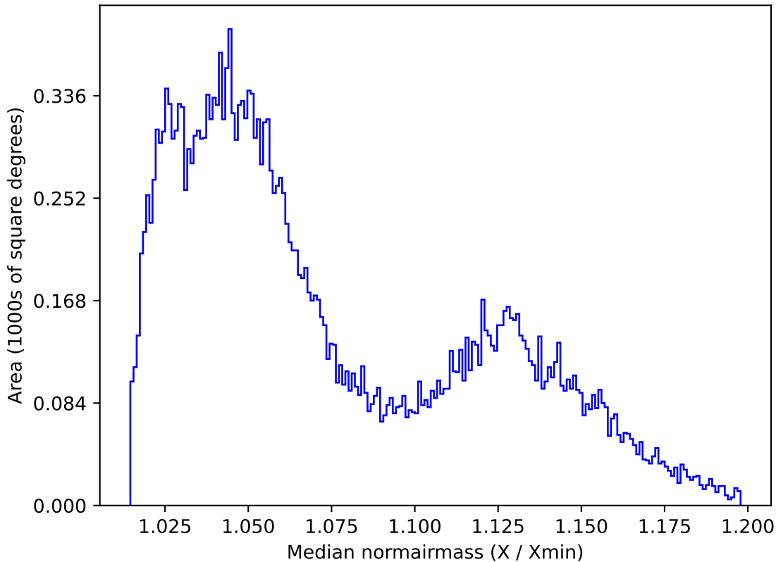
too_elab_r32_d3_giz_v3.4_10yrs All sky r band: Median normairmass
