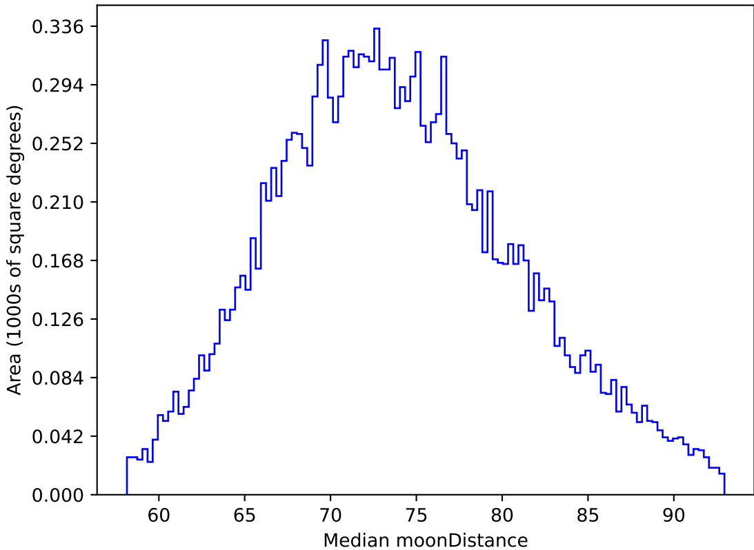
too_elab_r32_d3_giz_v3.4_10yrs WFD z band: Median moonDistance
