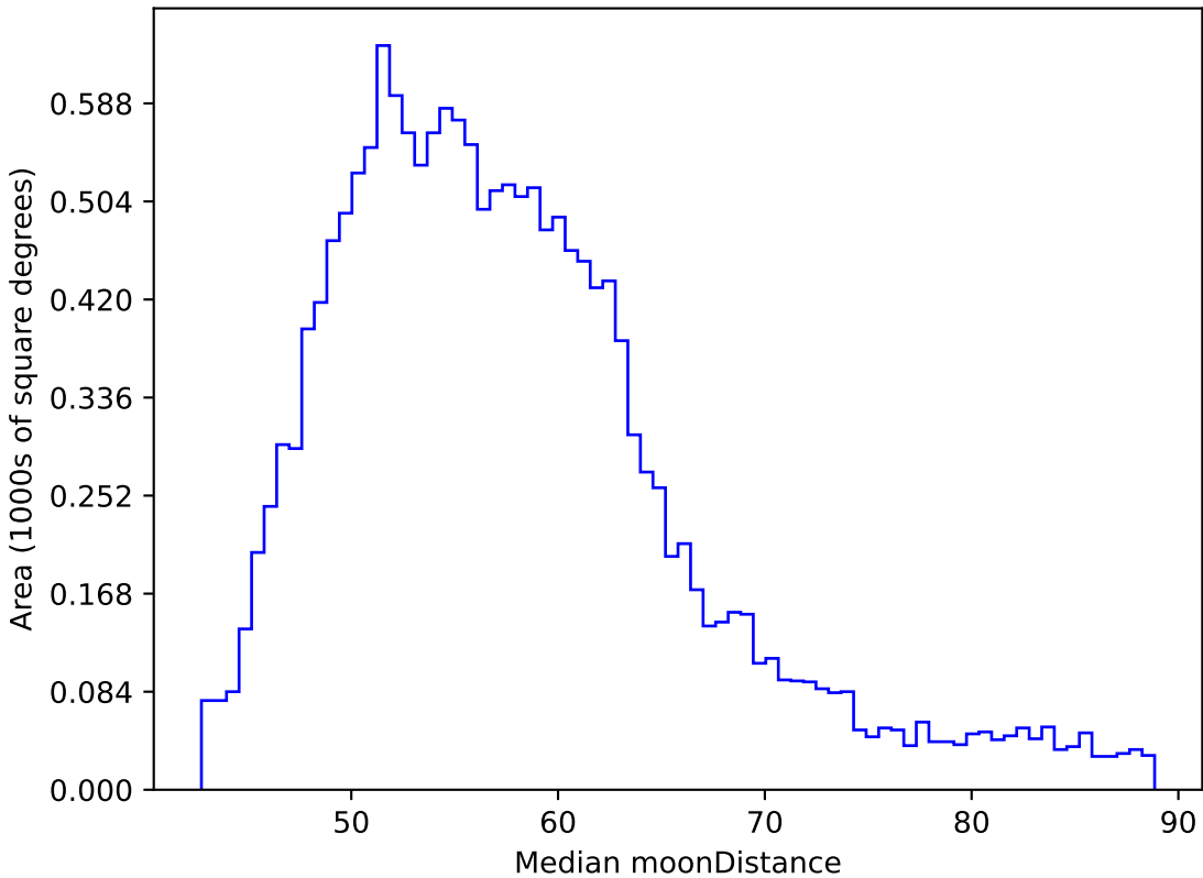
too_elab_r32_d3_giz_v3.4_10yrs WFD y band: Median moonDistance
