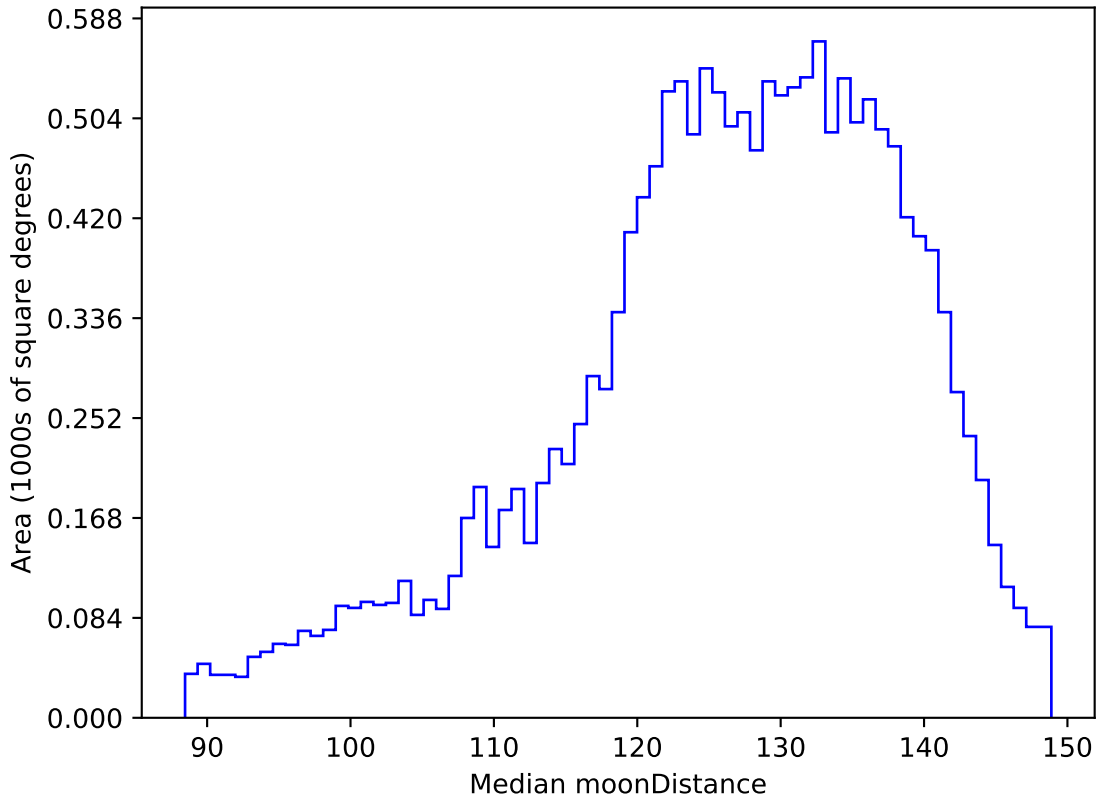
too_elab_r32_d3_giz_v3.4_10yrs WFD u band: Median moonDistance
