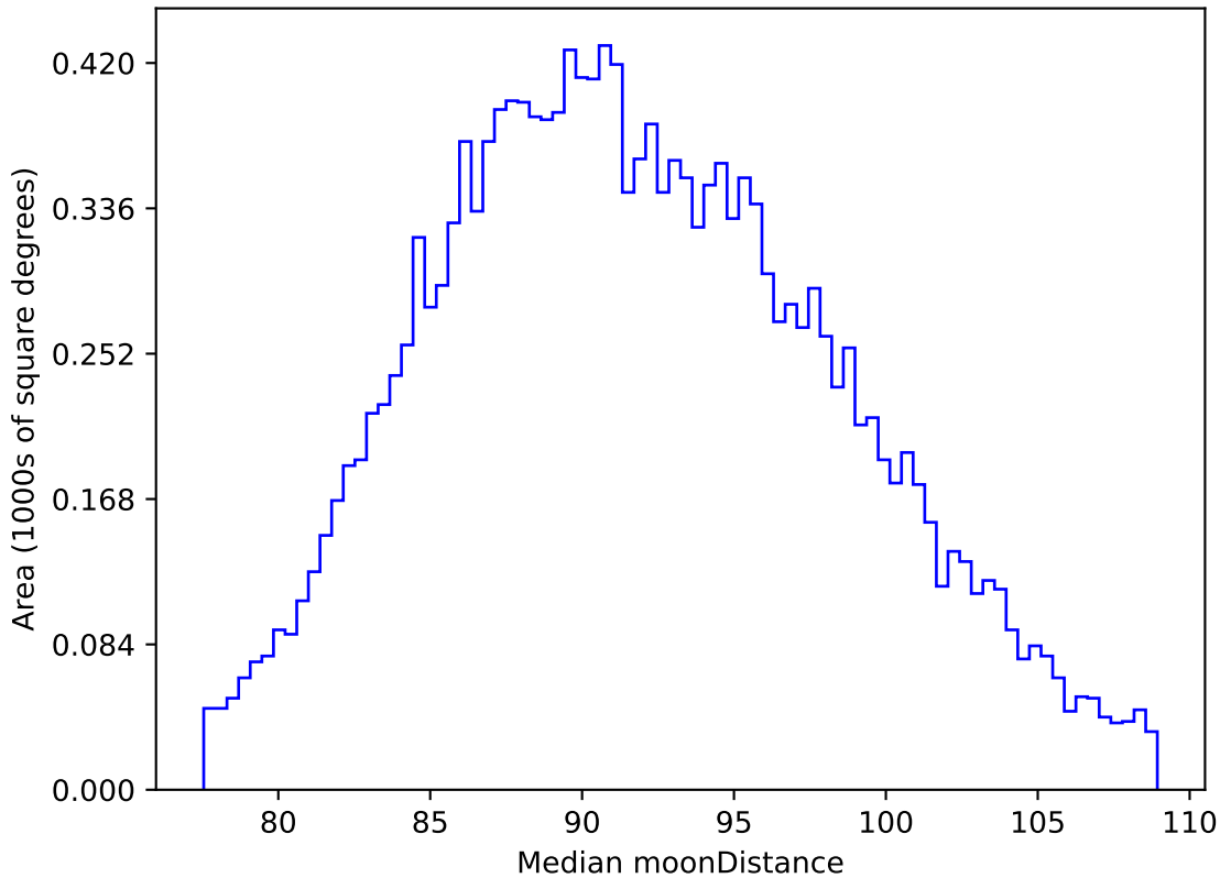
too_elab_r32_d3_giz_v3.4_10yrs WFD i band: Median moonDistance
