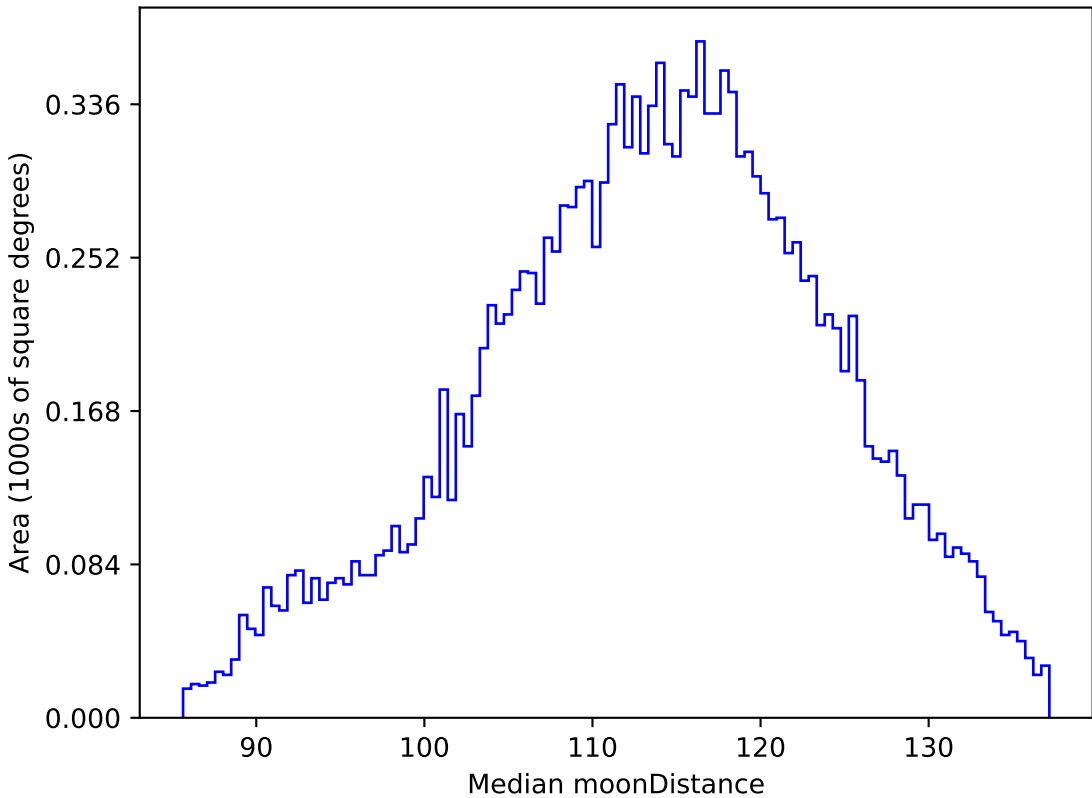
too_elab_r32_d3_giz_v3.4_10yrs WFD g band: Median moonDistance
