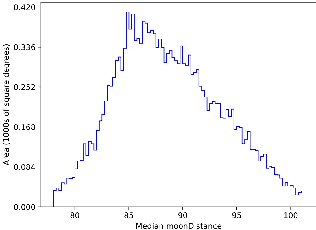
too_elab_r32_d3_giz_v3.4_10yrs WFD all bands: Median moonDistance
