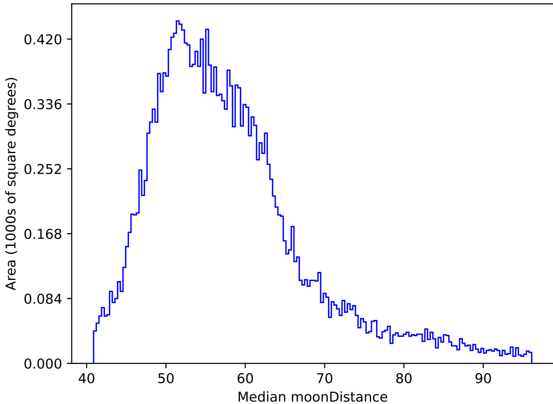
too_elab_r32_d3_giz_v3.4_10yrs All sky y band: Median moonDistance
