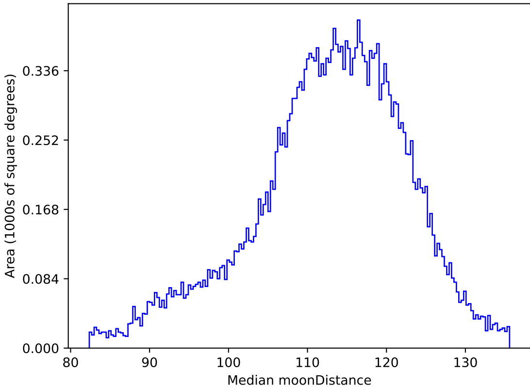
too_elab_r32_d3_giz_v3.4_10yrs All sky r band: Median moonDistance
