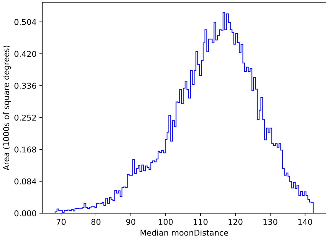
too_elab_r32_d3_giz_v3.4_10yrs All sky g band: Median moonDistance
