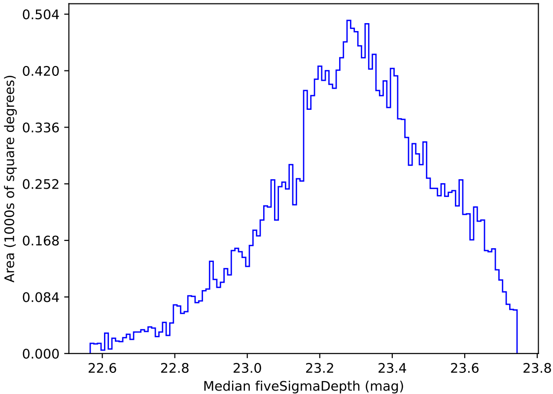
too_elab_r32_d3_giz_v3.4_10yrs Yr 1 u band: Median fiveSigmaDepth
