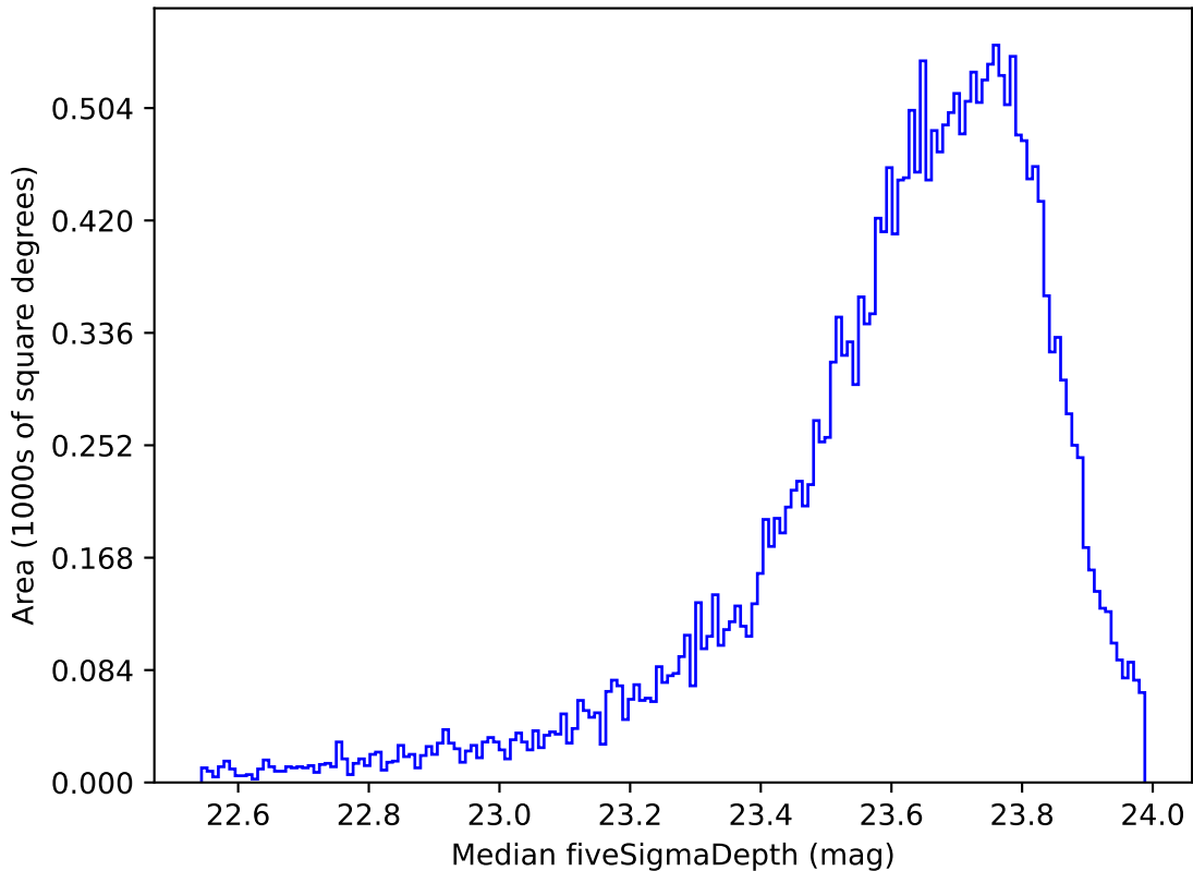
too_elab_r32_d3_giz_v3.4_10yrs Yr 1 i band: Median fiveSigmaDepth
