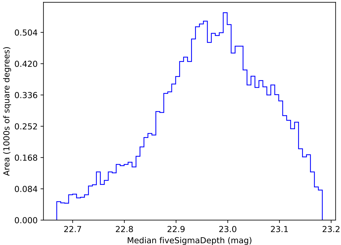
too_elab_r32_d3_giz_v3.4_10yrs WFD z band: Median fiveSigmaDepth
