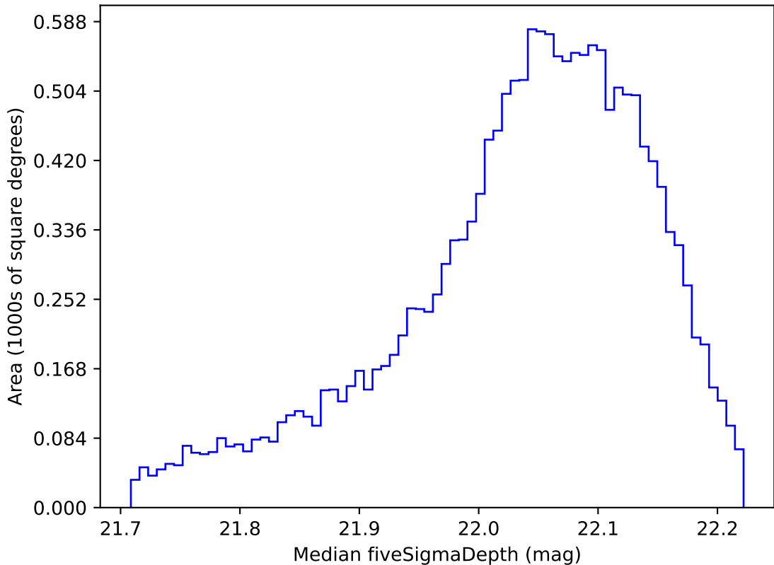
too_elab_r32_d3_giz_v3.4_10yrs WFD y band: Median fiveSigmaDepth
