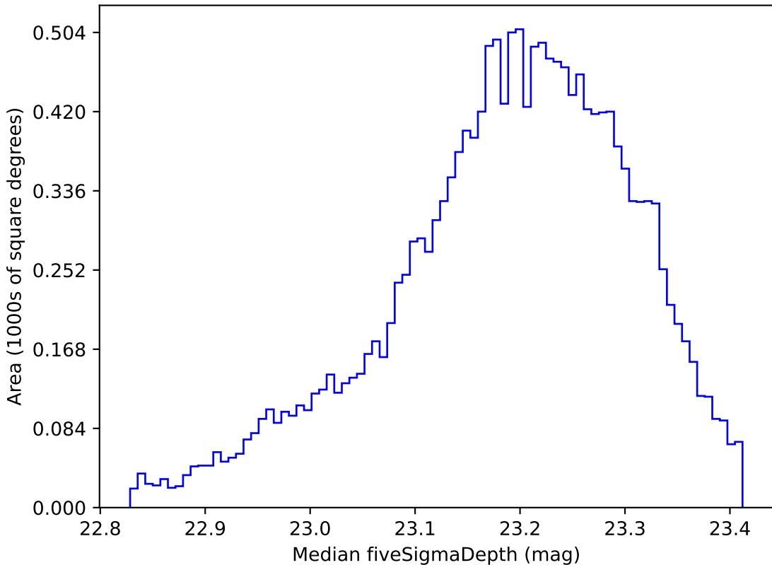
too_elab_r32_d3_giz_v3.4_10yrs WFD u band: Median fiveSigmaDepth
