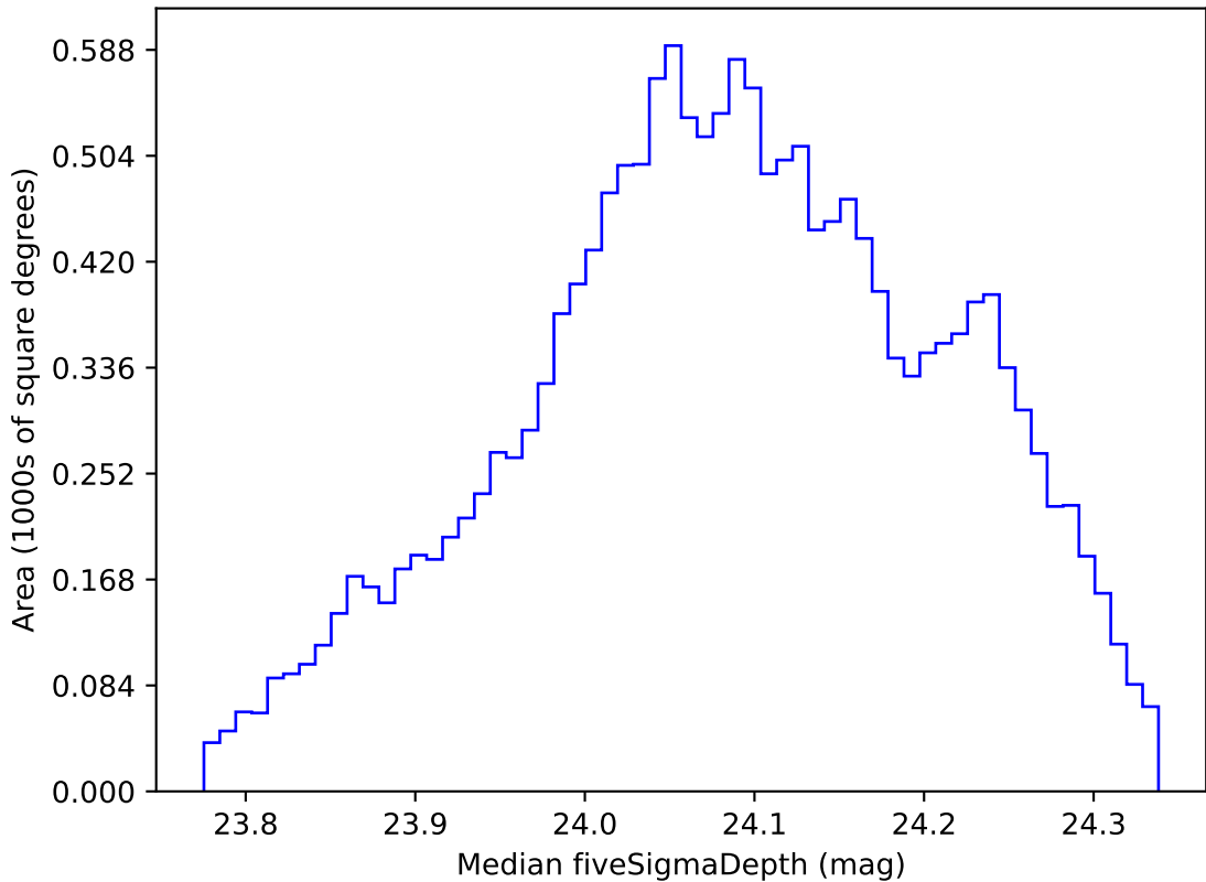
too_elab_r32_d3_giz_v3.4_10yrs WFD r band: Median fiveSigmaDepth
