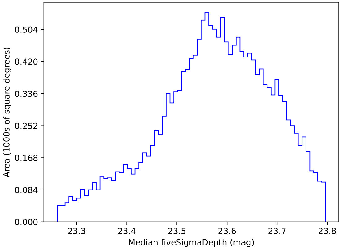
too_elab_r32_d3_giz_v3.4_10yrs WFD i band: Median fiveSigmaDepth
