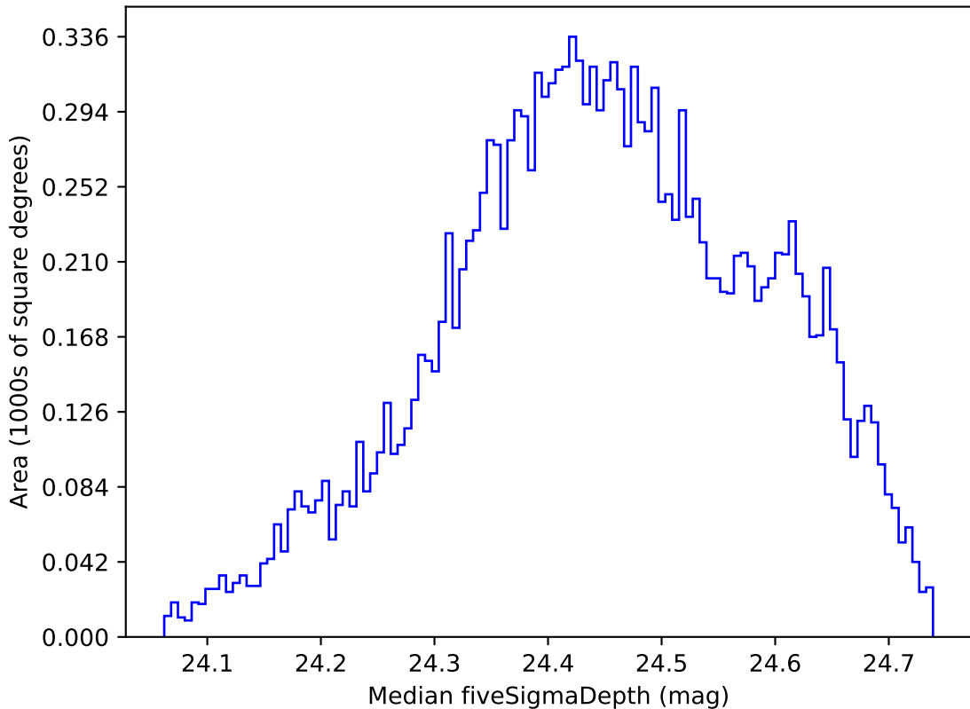
too_elab_r32_d3_giz_v3.4_10yrs WFD g band: Median fiveSigmaDepth
