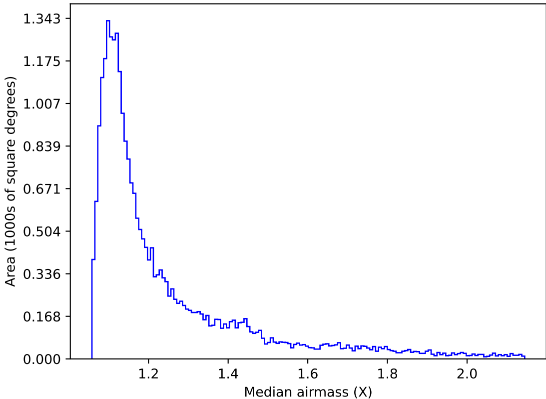
too_elab_r32_d3_giz_v3.4_10yrs Yr 1 r band: Median airmass
