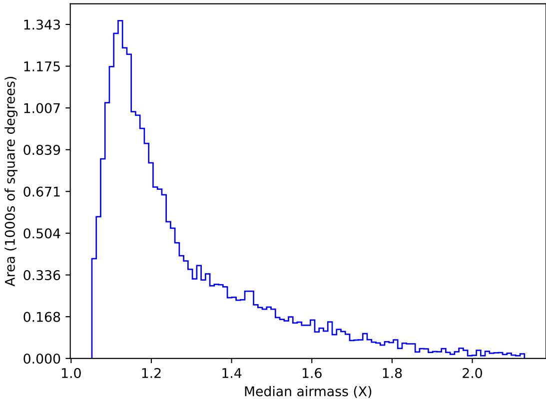
too_elab_r32_d3_giz_v3.4_10yrs Yr 1 g band: Median airmass
