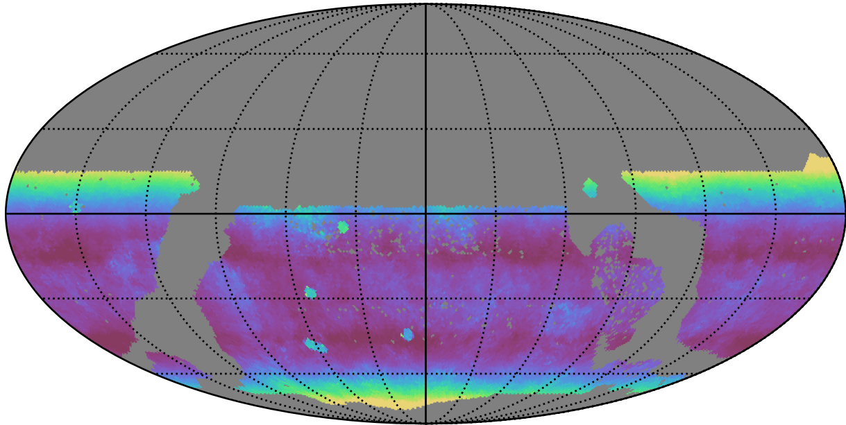
too_elab_r32_d3_giz_v3.4_10yrs WFD z band: Median airmass
