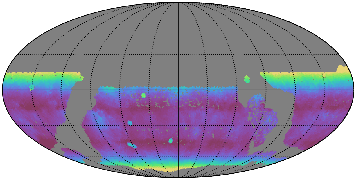
too_elab_r32_d3_giz_v3.4_10yrs WFD y band: Median airmass
