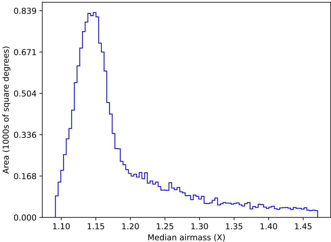
too_elab_r32_d3_giz_v3.4_10yrs WFD y band: Median airmass
