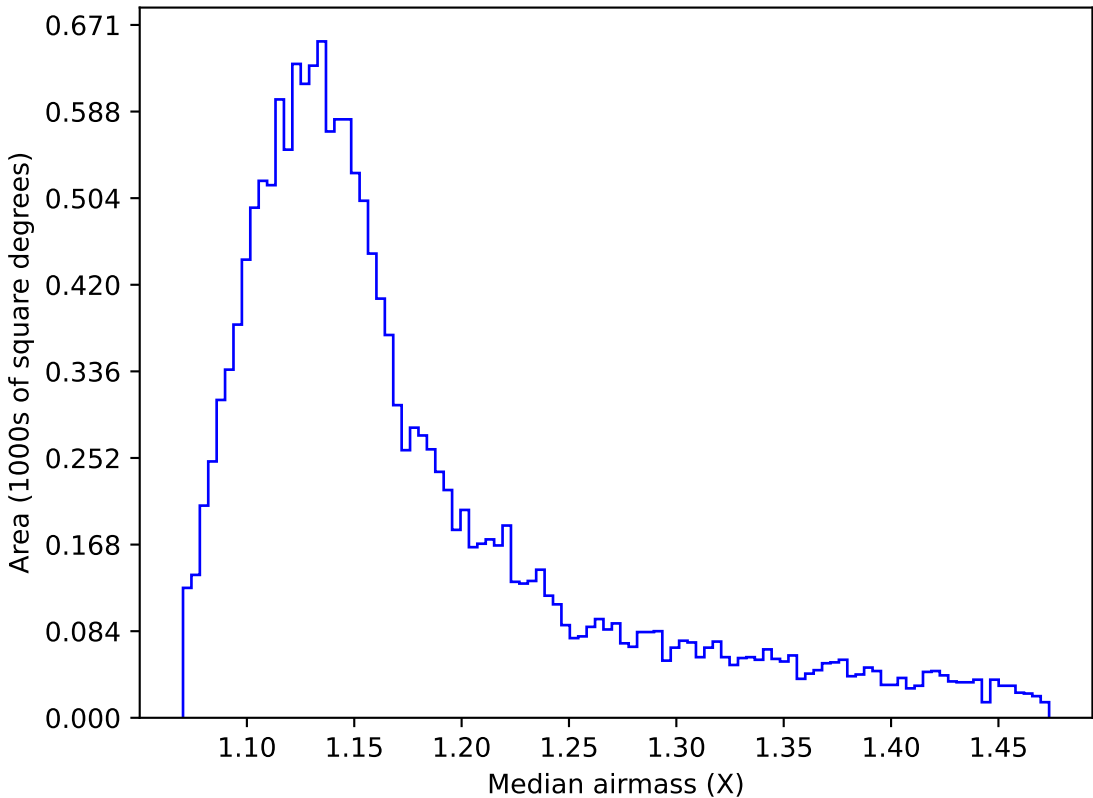
too_elab_r32_d3_giz_v3.4_10yrs WFD u band: Median airmass
