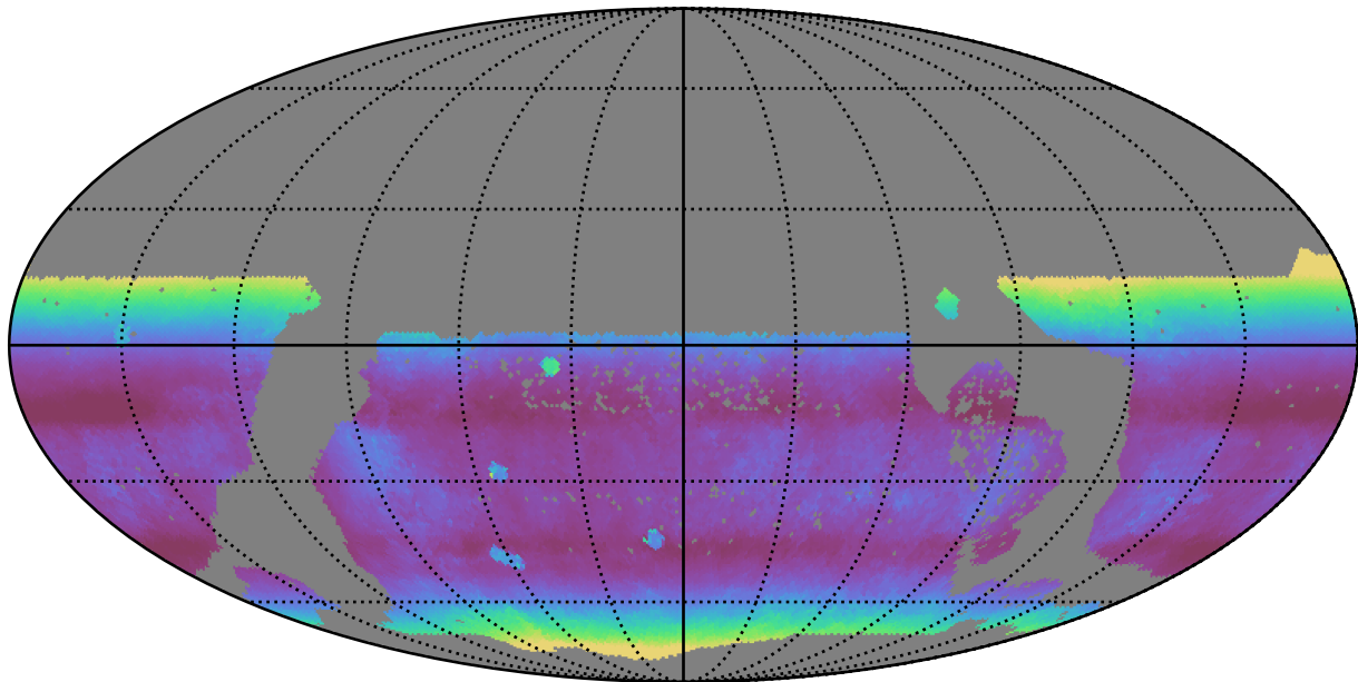
too_elab_r32_d3_giz_v3.4_10yrs WFD r band: Median airmass
