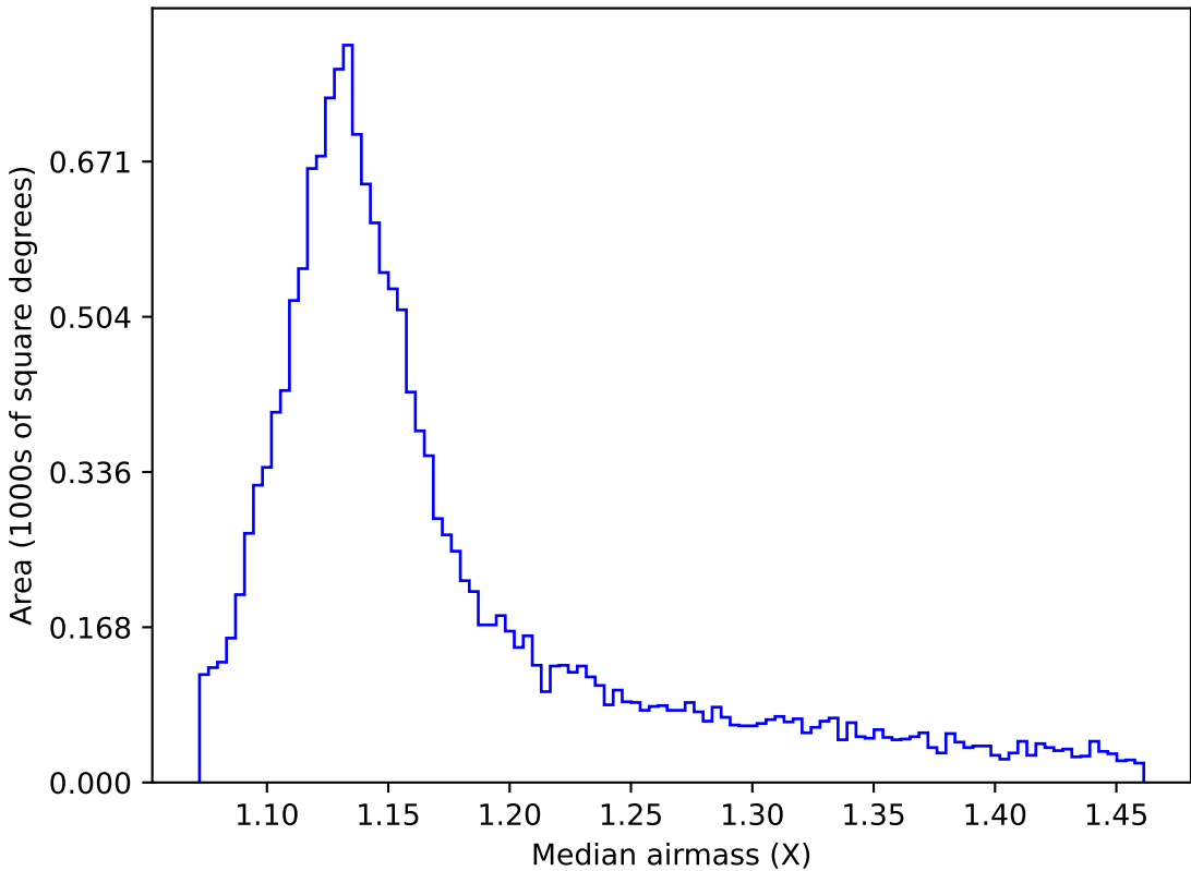
too_elab_r32_d3_giz_v3.4_10yrs WFD r band: Median airmass
