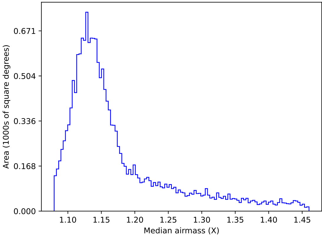
too_elab_r32_d3_giz_v3.4_10yrs WFD i band: Median airmass
