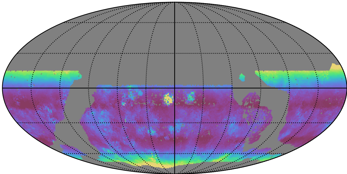
too_elab_r32_d3_giz_v3.4_10yrs WFD g band: Median airmass
