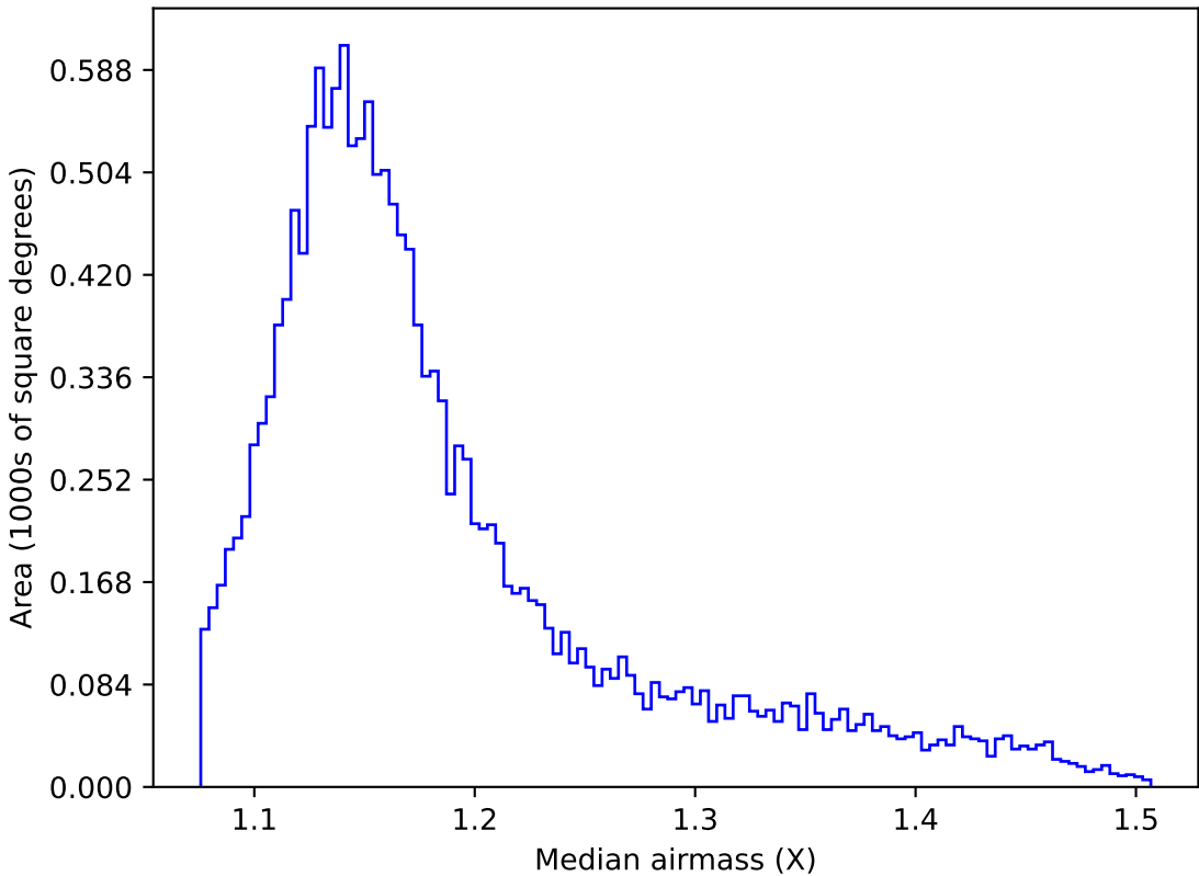
too_elab_r32_d3_giz_v3.4_10yrs WFD g band: Median airmass
