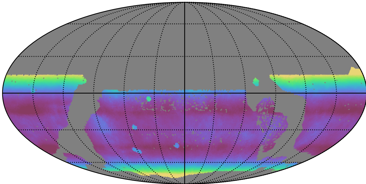
too_elab_r32_d3_giz_v3.4_10yrs WFD all bands: Median airmass
