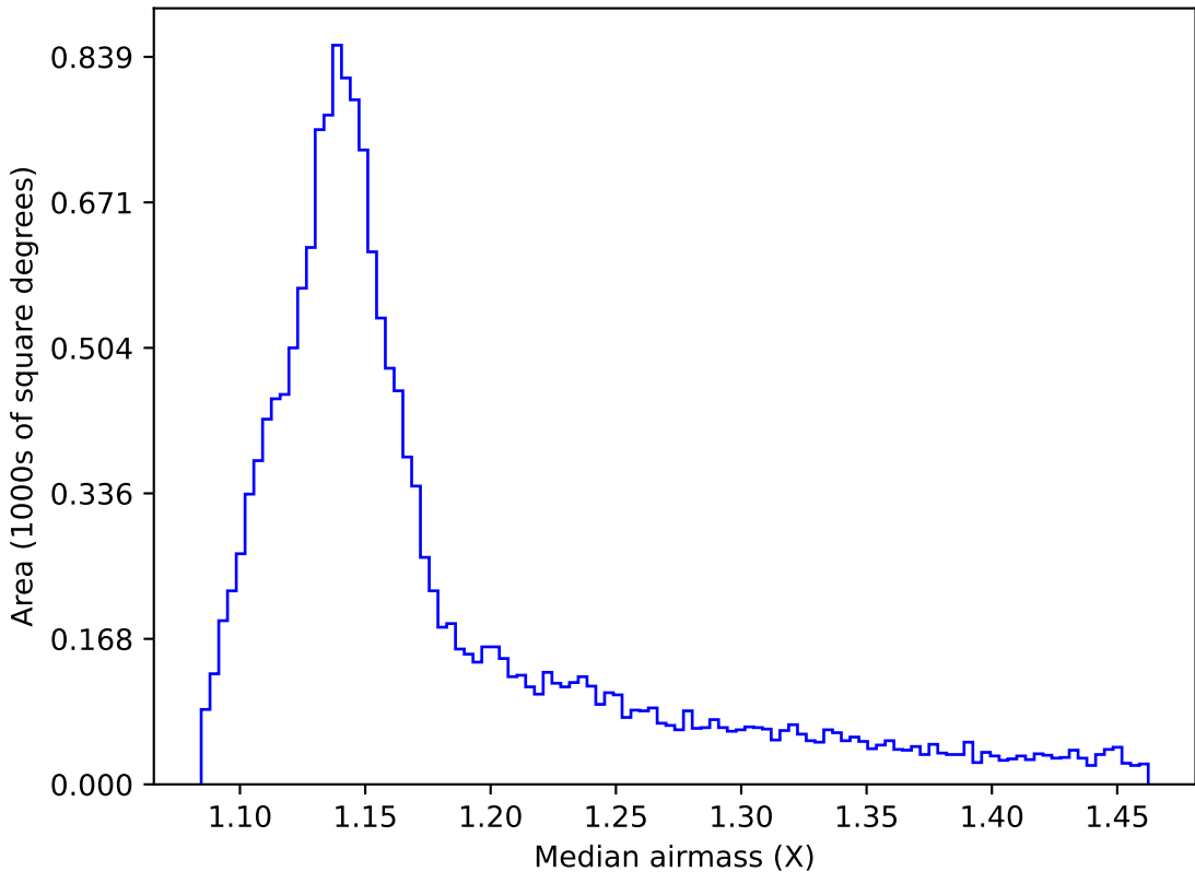
too_elab_r32_d3_giz_v3.4_10yrs WFD all bands: Median airmass
