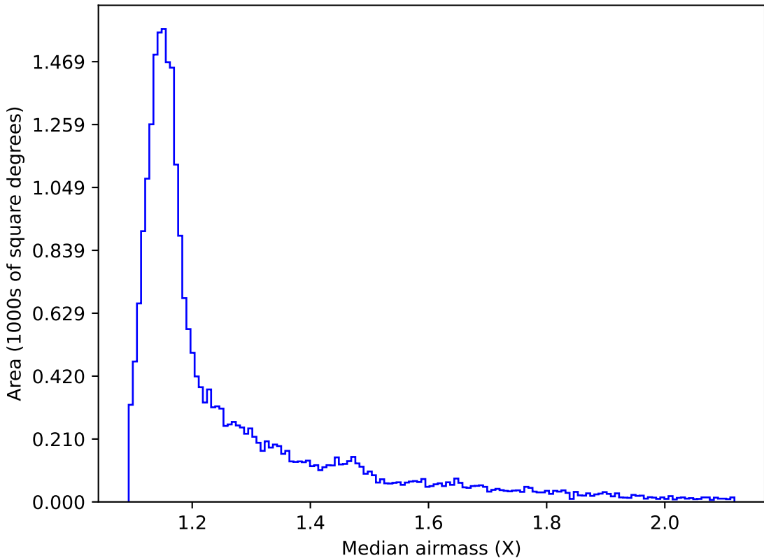
too_elab_r32_d3_giz_v3.4_10yrs All sky z band: Median airmass
