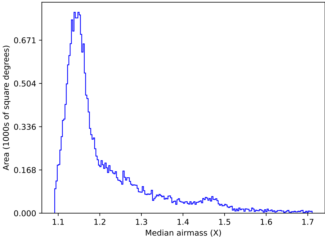
too_elab_r32_d3_giz_v3.4_10yrs All sky y band: Median airmass
