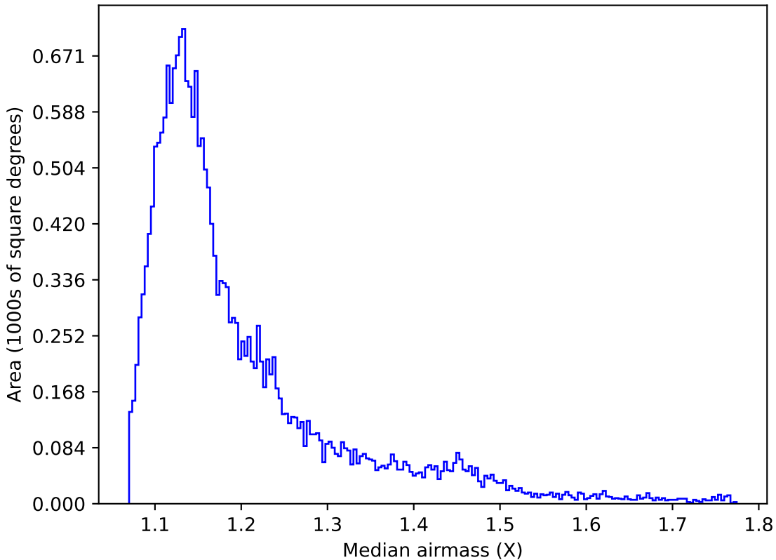
too_elab_r32_d3_giz_v3.4_10yrs All sky u band: Median airmass
