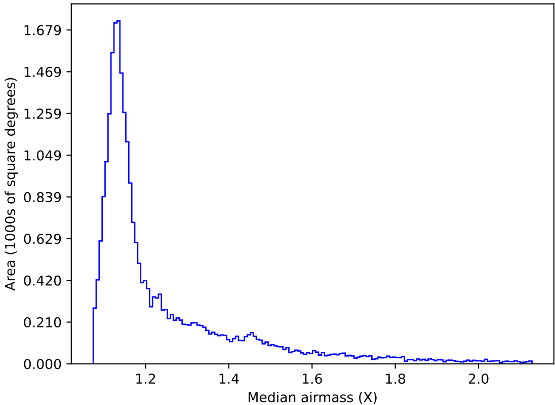
too_elab_r32_d3_giz_v3.4_10yrs All sky r band: Median airmass
