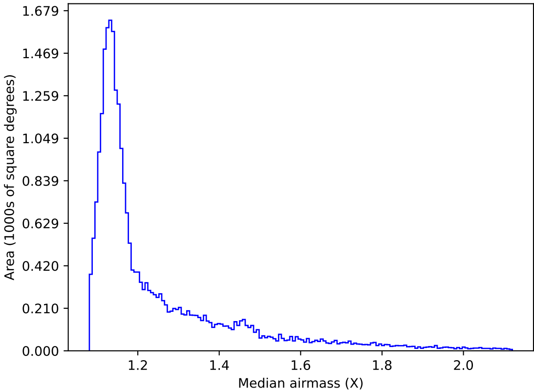
too_elab_r32_d3_giz_v3.4_10yrs All sky i band: Median airmass
