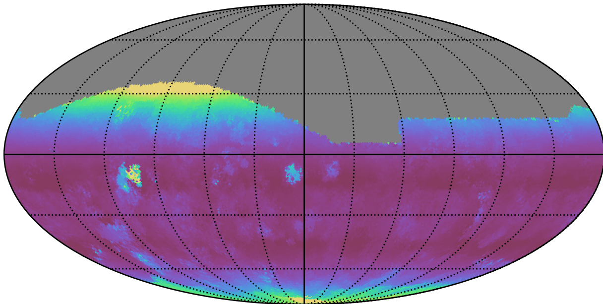
too_elab_r32_d3_giz_v3.4_10yrs All sky g band: Median airmass
