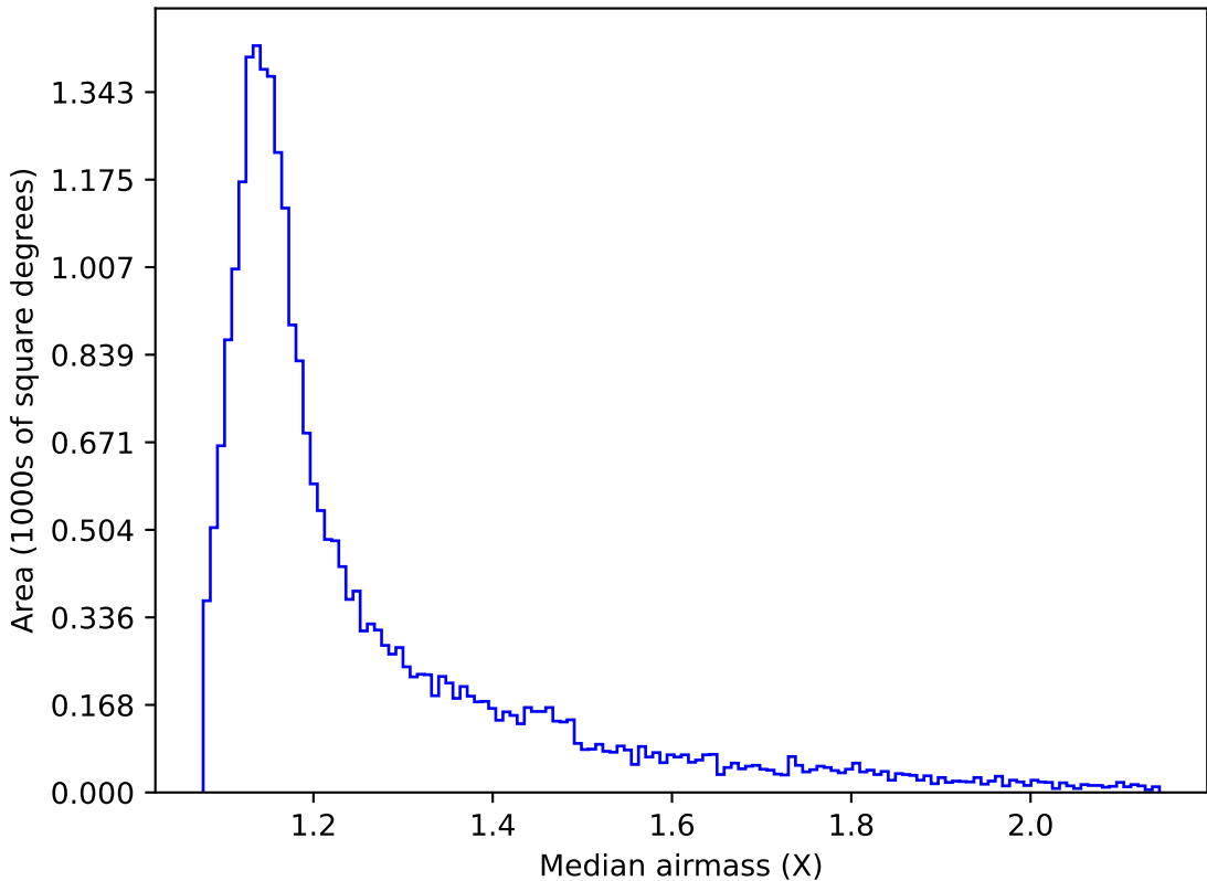
too_elab_r32_d3_giz_v3.4_10yrs All sky g band: Median airmass
