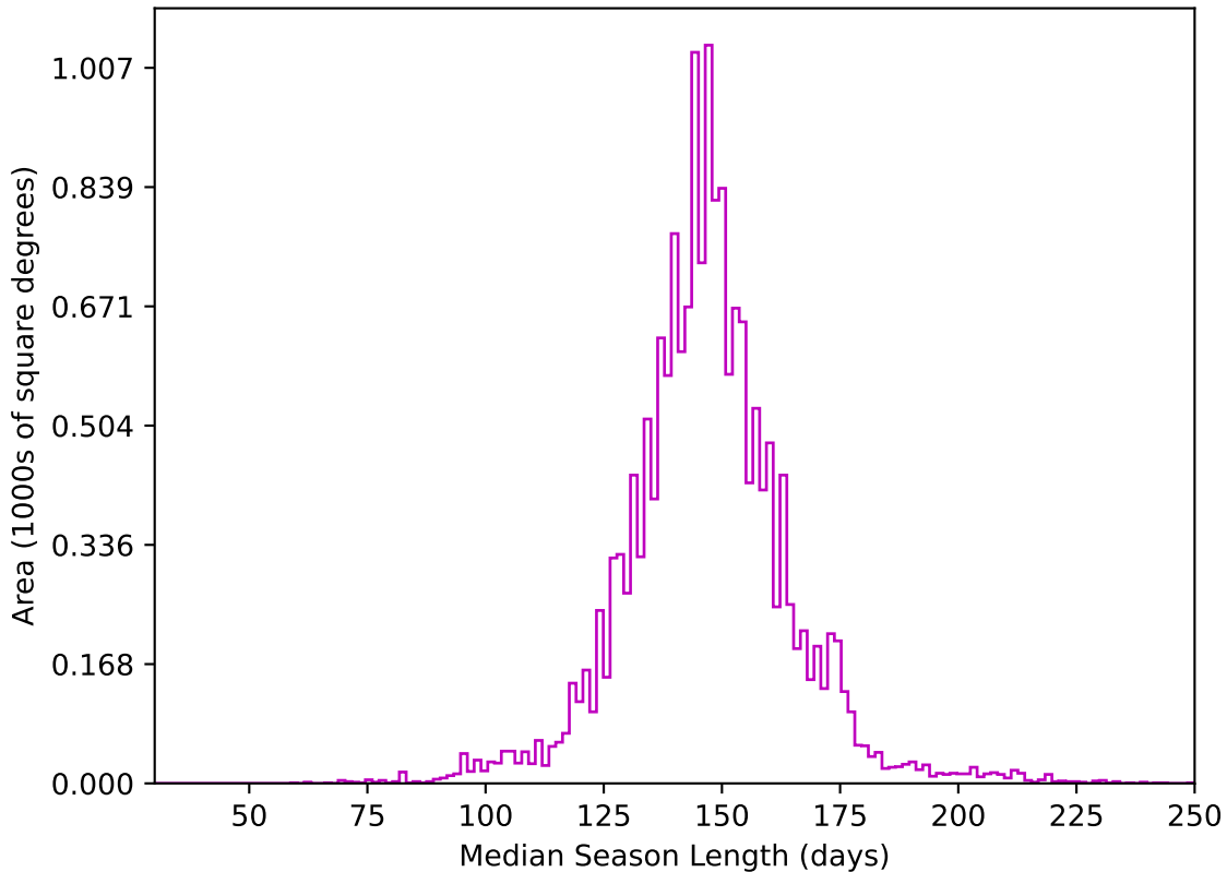
too_elab_r32_d3_giz_v3.4_10yrs WFD z band: Median Season Length
