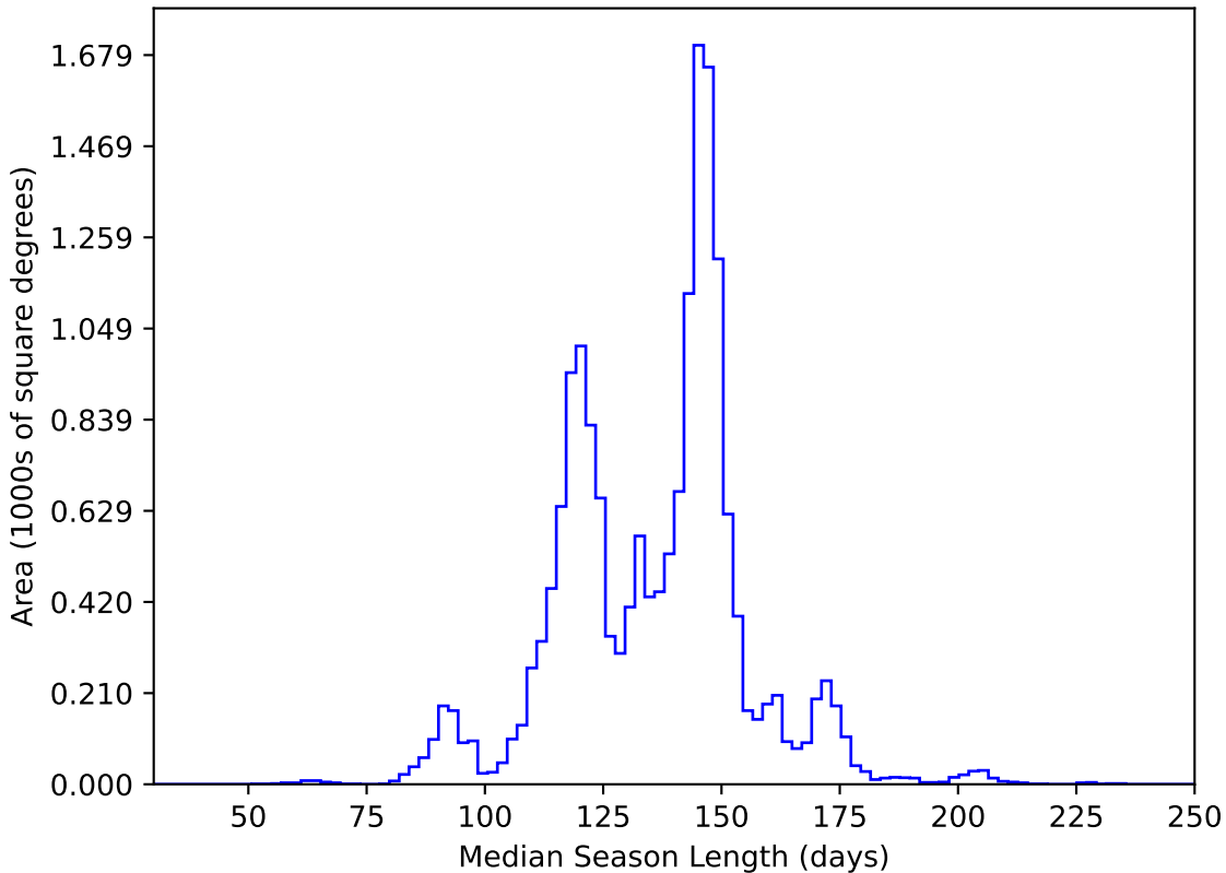
too_elab_r32_d3_giz_v3.4_10yrs WFD y band: Median Season Length
