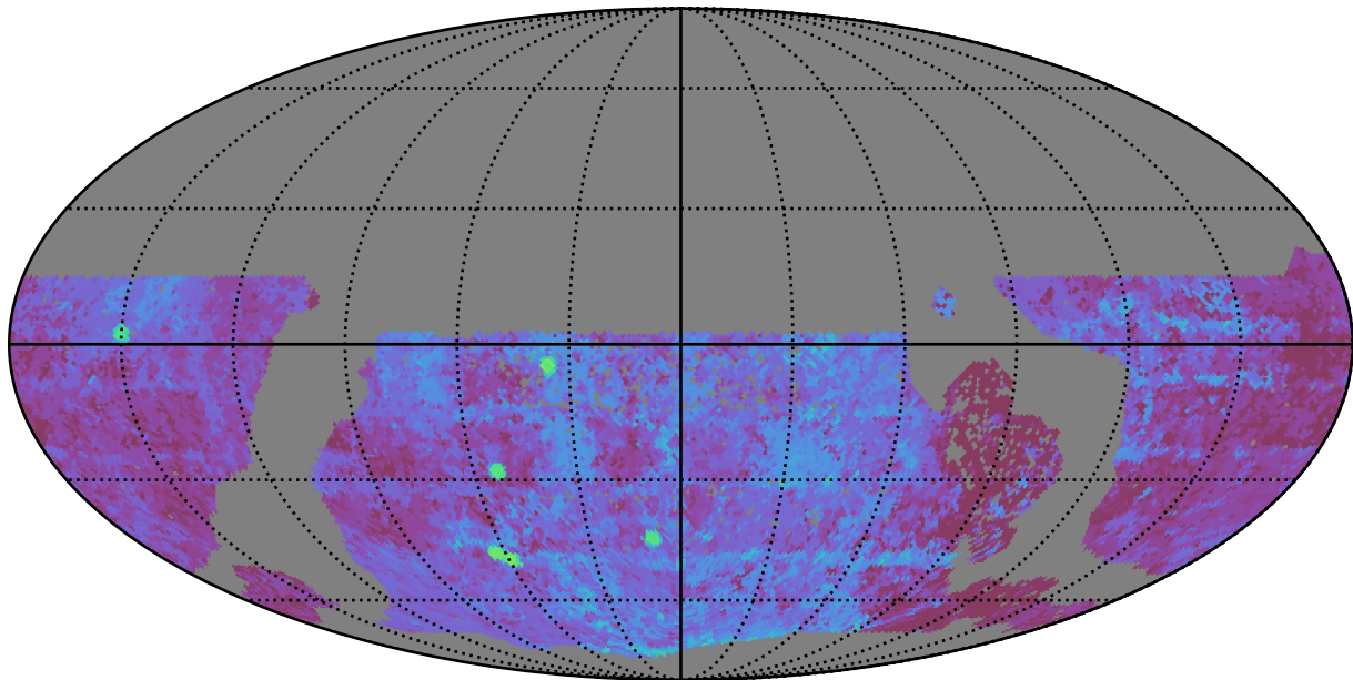
too_elab_r32_d3_giz_v3.4_10yrs WFD u band: Median Season Length
