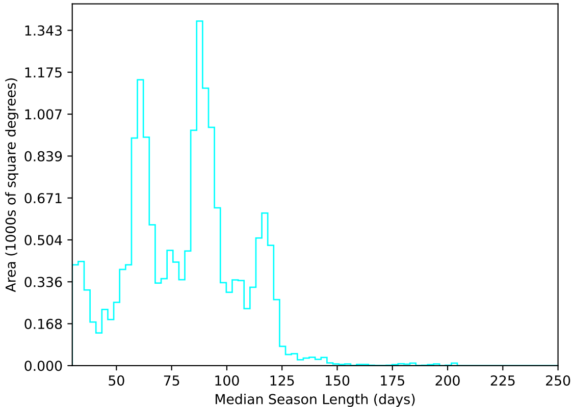
too_elab_r32_d3_giz_v3.4_10yrs WFD u band: Median Season Length
