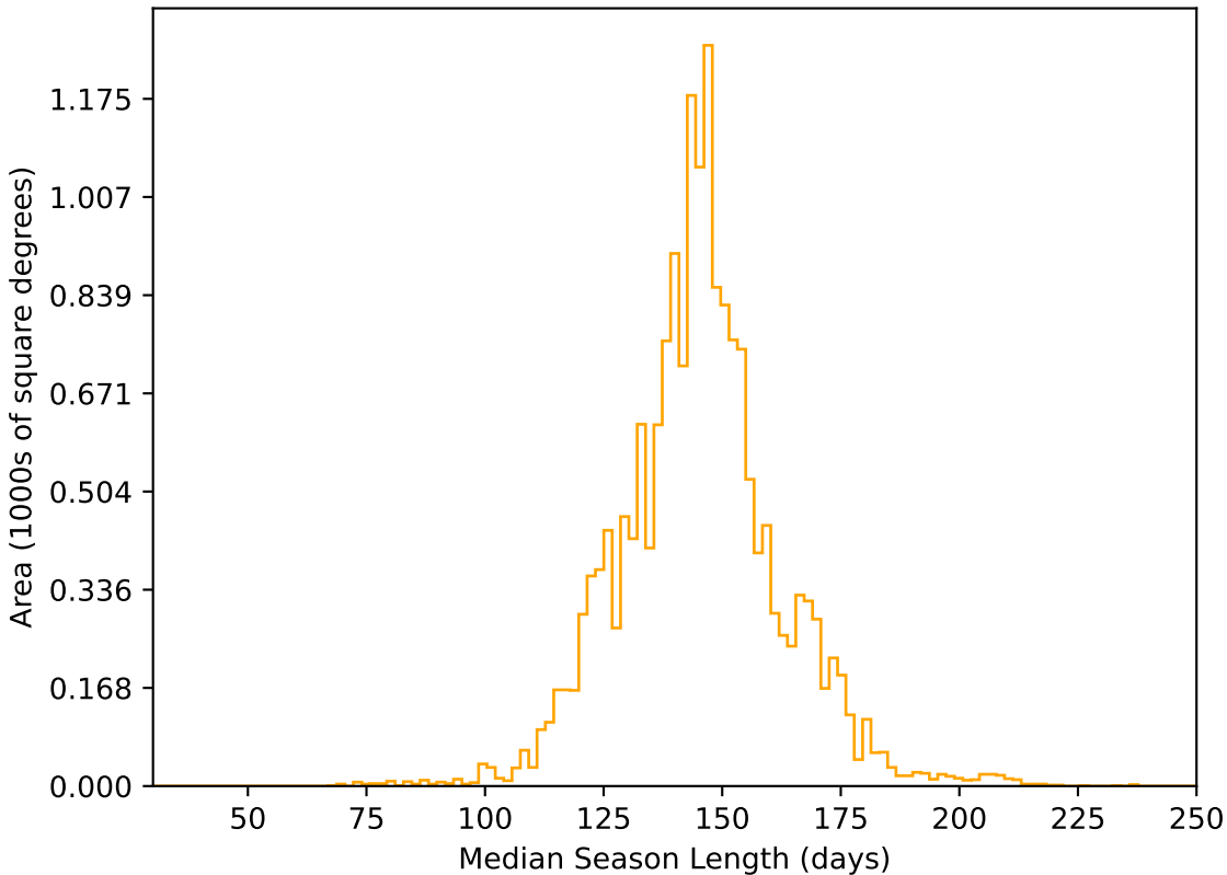
too_elab_r32_d3_giz_v3.4_10yrs WFD r band: Median Season Length
