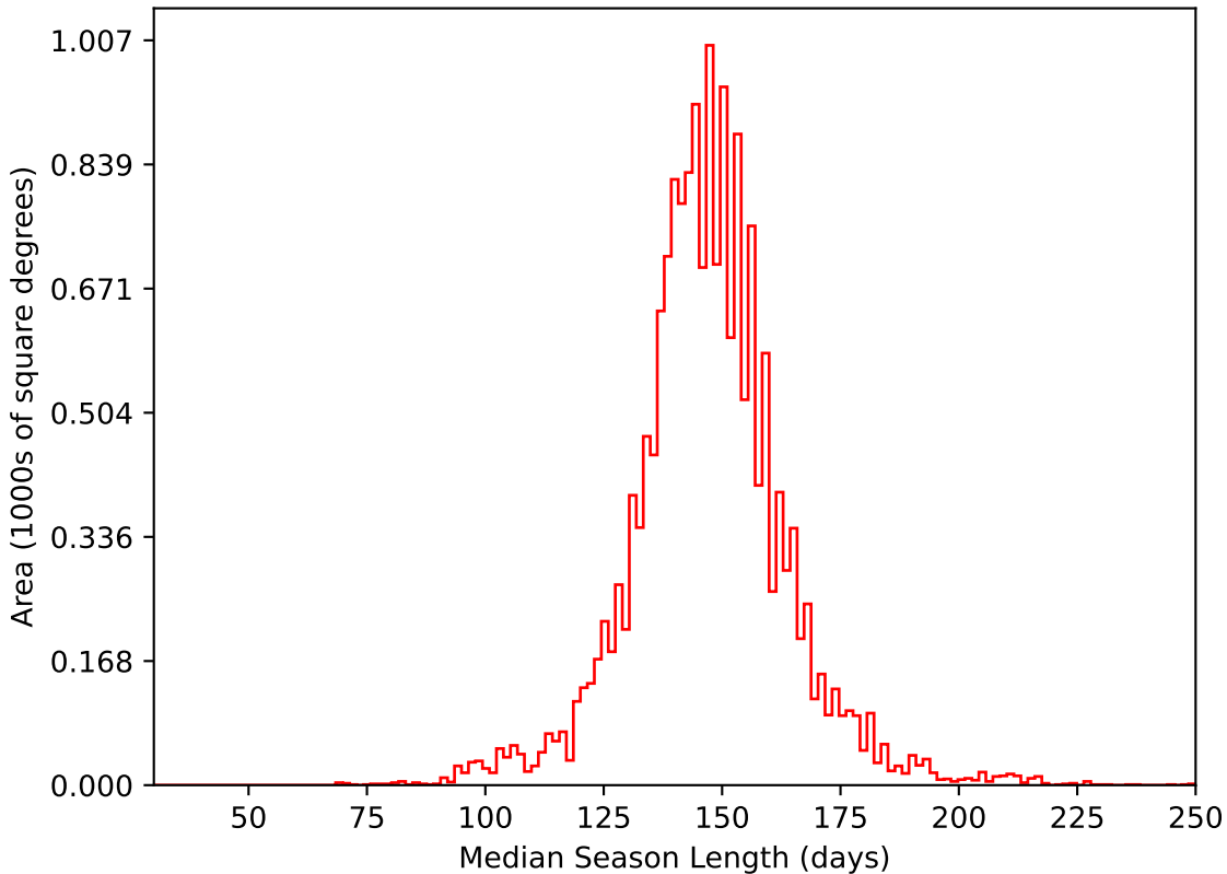
too_elab_r32_d3_giz_v3.4_10yrs WFD i band: Median Season Length
