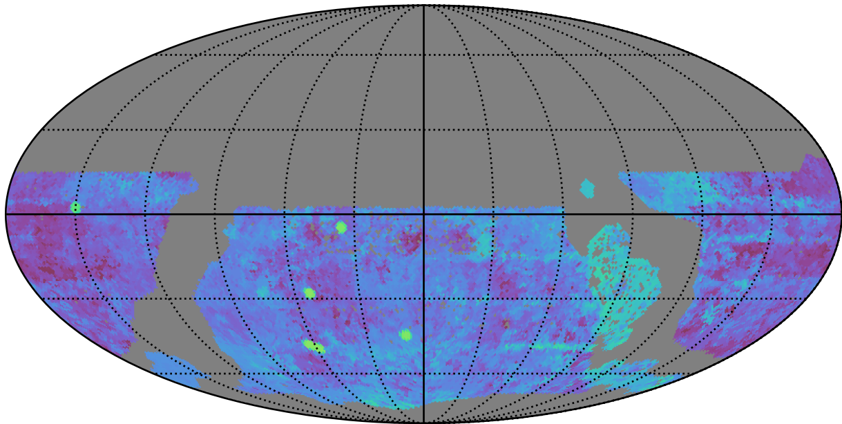
too_elab_r32_d3_giz_v3.4_10yrs WFD g band: Median Season Length
