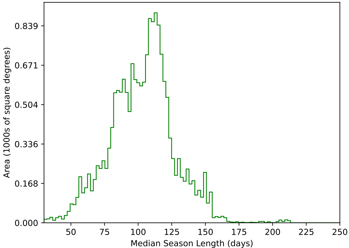
too_elab_r32_d3_giz_v3.4_10yrs WFD g band: Median Season Length
