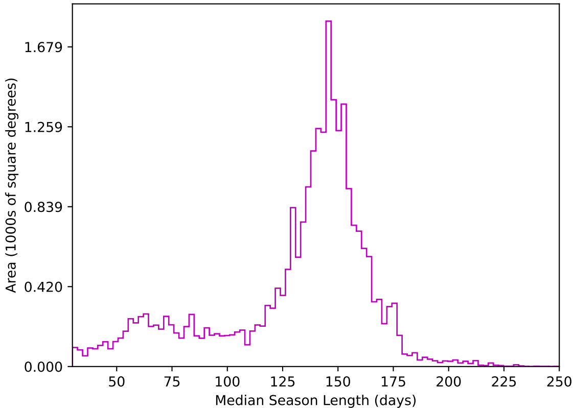
too_elab_r32_d3_giz_v3.4_10yrs All sky z band: Median Season Length
