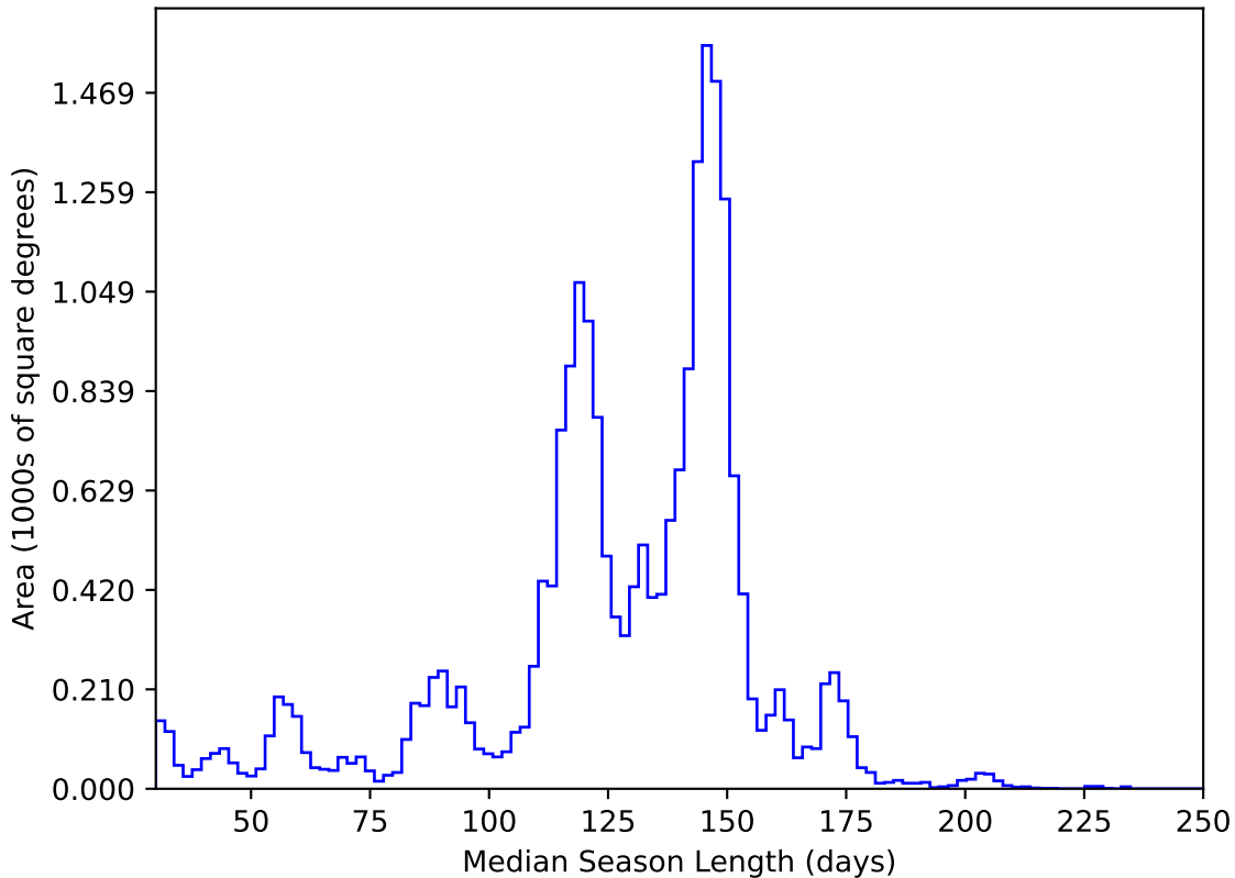
too_elab_r32_d3_giz_v3.4_10yrs All sky y band: Median Season Length
