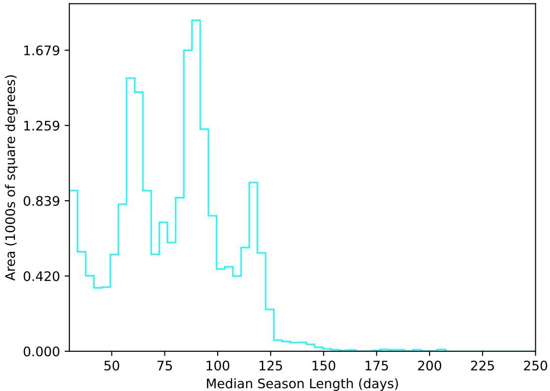
too_elab_r32_d3_giz_v3.4_10yrs All sky u band: Median Season Length
